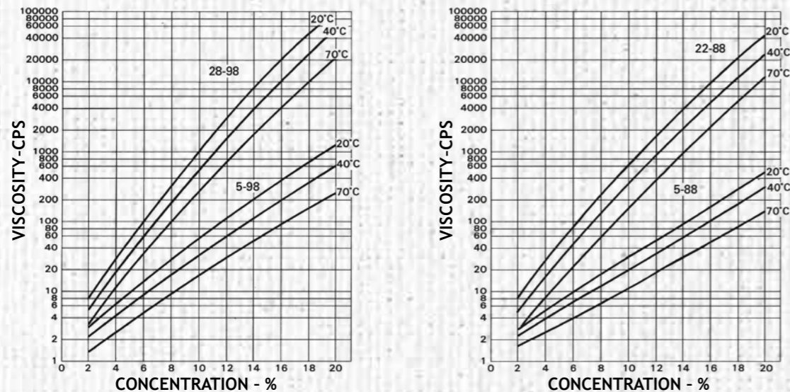
Figure 2: Viscosity Concentration Relationship for Aqueous Solutions of KURARAY POVAL™ at Various Temperature
