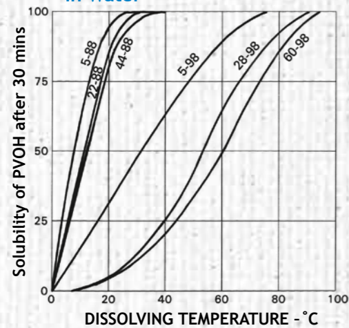
Figure 1: Dissolving Rate of KURARAY POVAL™ in Water
