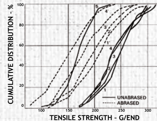
Residual Strength of Sized Yarn after Abrasions by Stationary Weaving
